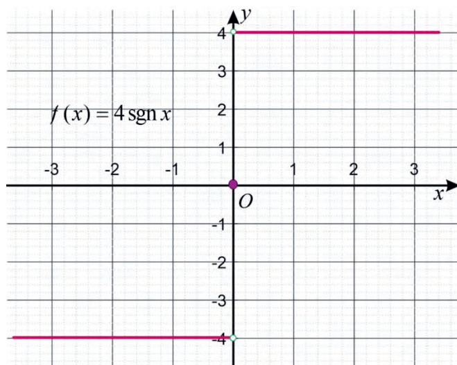
Figure 1.48: Graph of f(x) = 4\operatorname{sgn} x
