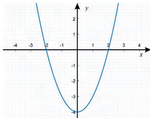
Figure 1.15: Graph of a relation S
