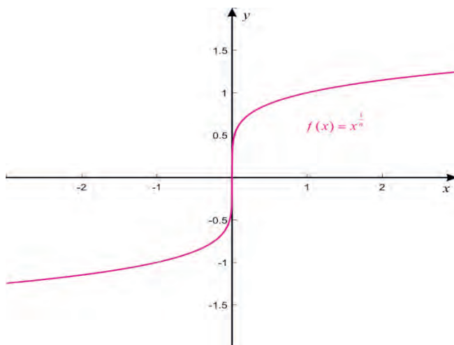
Figure 1.27: Graph of f(x) = x^{\frac{1}{n}} , where n is an odd natural number.
