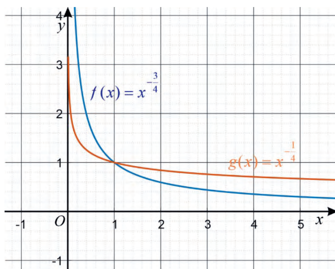
Figure 1.32: Graphs of f(x) = x^{-\frac{3}{4}} and g(x) = x^{-\frac{1}{4}}
