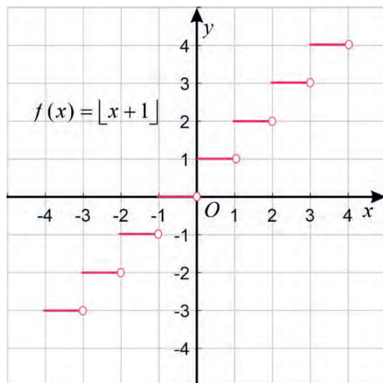
Figure 1.51: Graph of f(x) = \lfloor x + 1 \rfloor .
