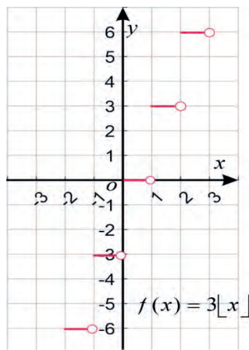
Figure 1.52: Graph of f(x) = 3[x]
