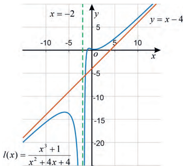
Figure 2.5: Graph of l(x) = \frac{x^3 + 1}{x^2 + 4x + 4}
