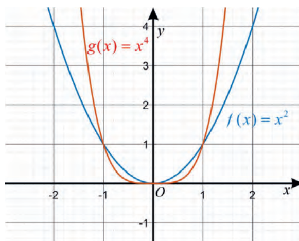
Figure 1.20: Graphs of f(x) = x^2 and g(x) = x^4
