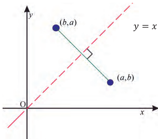
Figure 1.9: Image of (a, b) with respect to the reflection on the line y = x .
