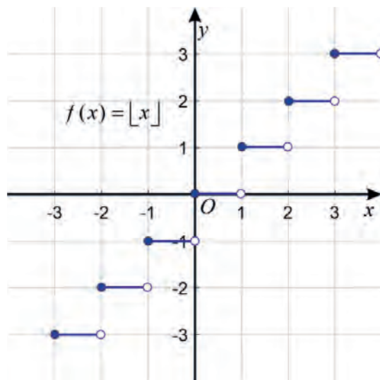
Figure 1.49: Graph of f(x) = \lfloor x \rfloor
