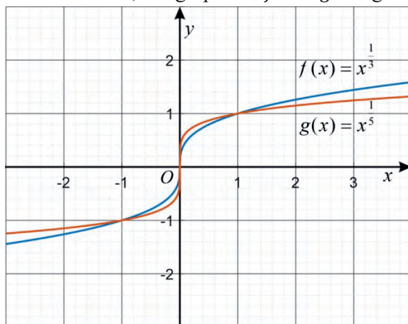
Figure 1.26: Graphs of f(x) = x^{\frac{1}{3}} and g(x) = x^{\frac{1}{5}}
