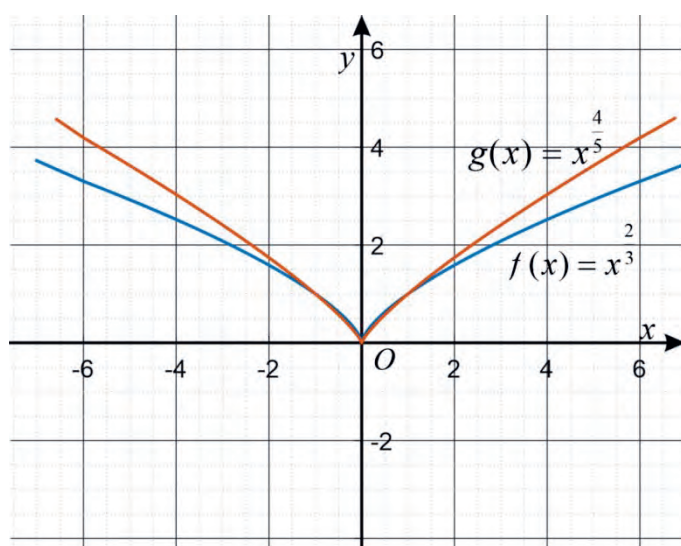
Figure 1.30: Graphs of f(x) = x^{\frac{2}{3}} and g(x) = x^{\frac{4}{5}}
