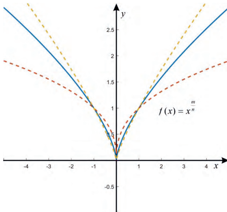
Figure 1.31: Graph of f(x) = x^{\frac{m}{n}} for an even natural number m and an odd natural number n
