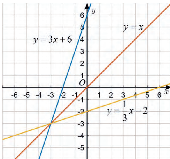
Figure 1.11: Graphs of y = 3x + 6 and y = \frac{1}{3}x - 2 .
