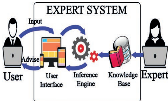
Figure 2.5 Expert system
