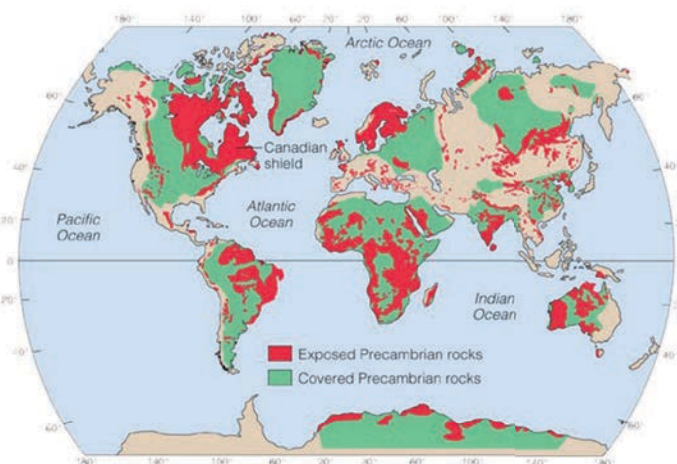
Figure 1.7 Distribution of Precambrian rocks (shields) [Wicander & Mon-
