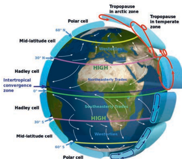
Figure 2.7: Global atmospheric circulation
