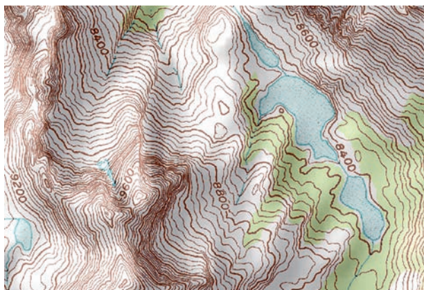
Figure 8.3. Contours represent major landform reliefs
