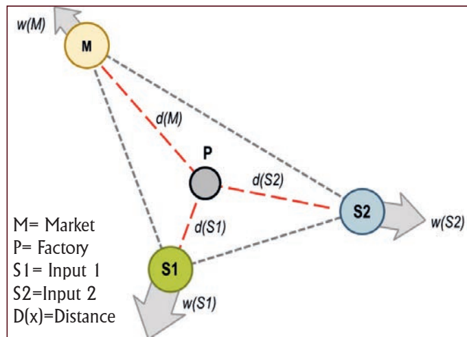
Figure 5.2 Weber's least cost triangular location model
