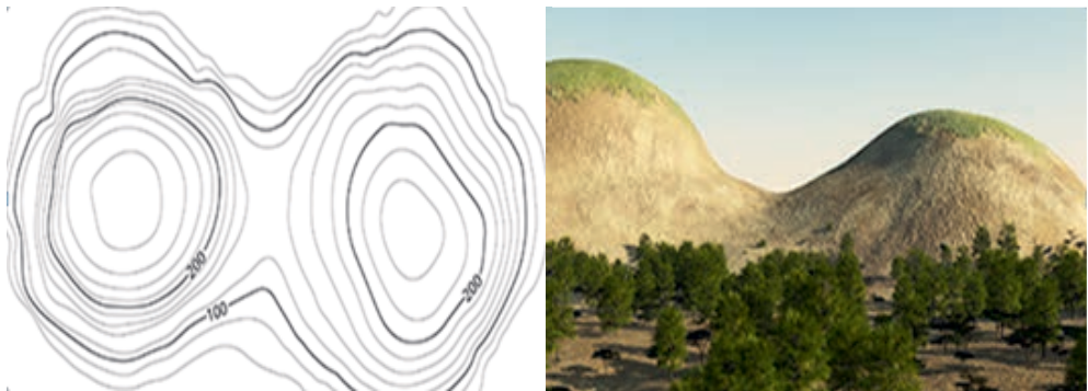
Figure: 8.7. Saddle contours
