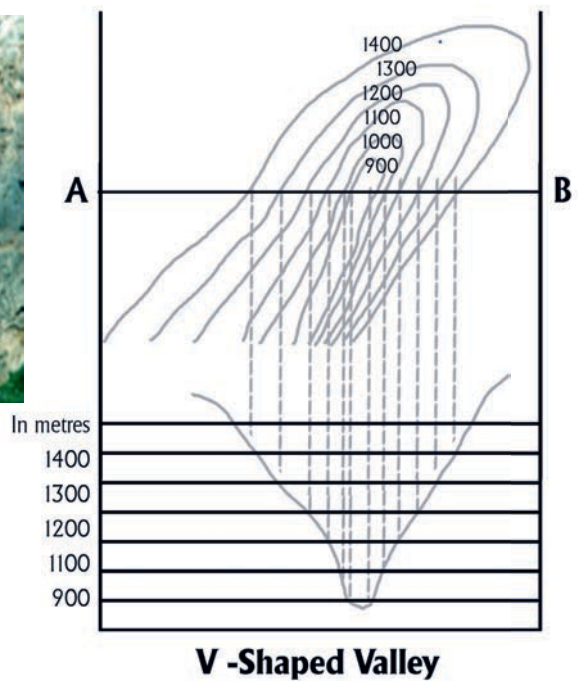
Figure: 8.6. Valley contours
