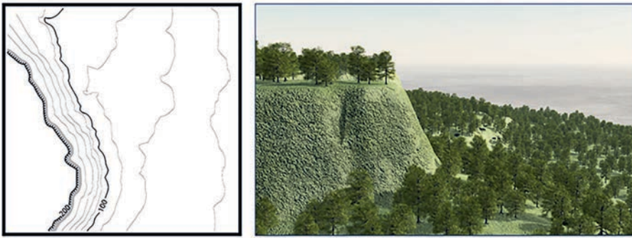
Figure 8.11. Spur contours
