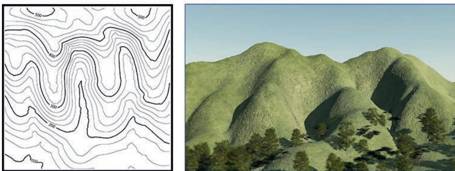
Figure 8.10. Spur contours
