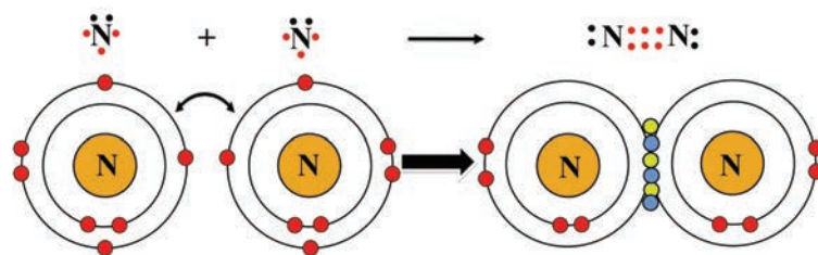
Figure 5.12 Atomic diagram of the formation of nitrogen molecule ( \text{N}_2 ).
