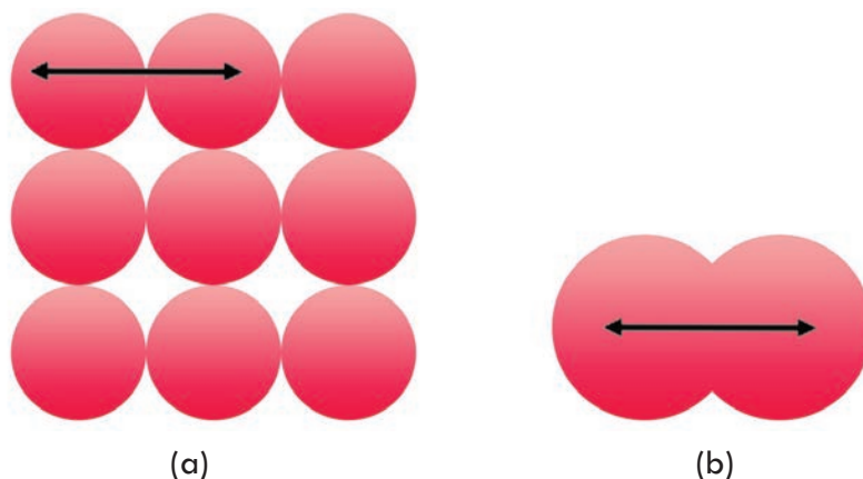
Figure 4.5 (a) In metals such as beryllium, the atomic radius is defined as one-half the distance between the centers of two adjacent atoms. (b) For elements that exist as diatomic molecules, such as iodine, the radius of the atom is defined as one-half the distance between the centers of the atoms in the molecule.
