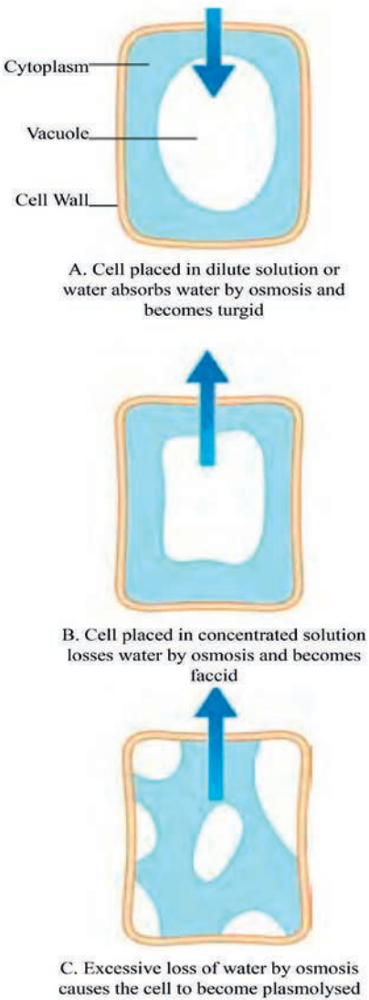
Fig. 3.16. Osmosis in plant
