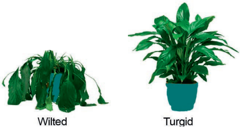
Figure 3.17. The effect of osmosis in plant leaf
