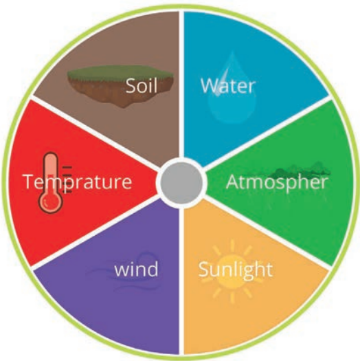
Figure 6.1. Common abiotic factors of territorial and aquatic biome
