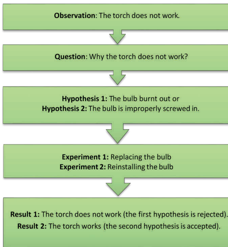
Figure 1.1. Application of the scientific method to common problems in our surroundings
