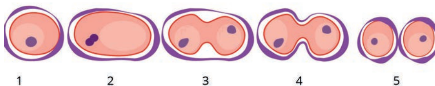
Figure 4.2. Binary fission in bacteria
