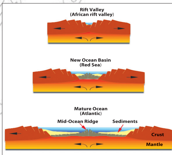
Figure 2.7 Formation of a rift valley
