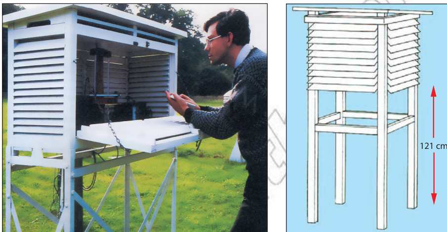
Figure 2.30 Stevenson screen
