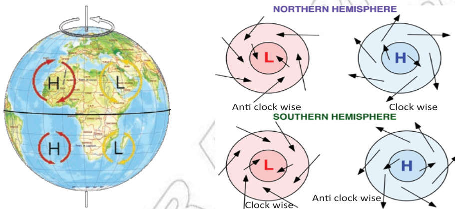
Figure 2.40 Cyclones and anticyclones
