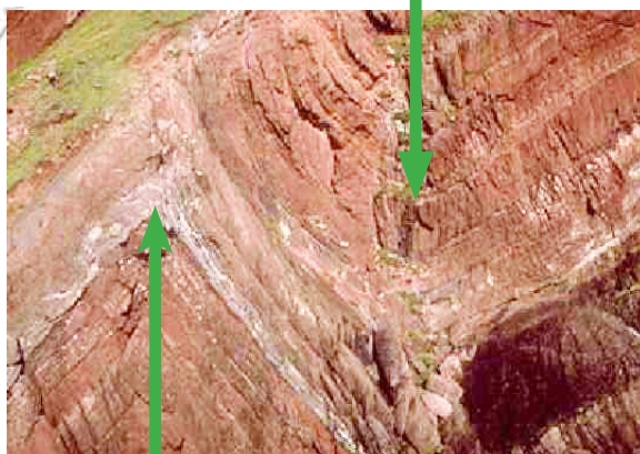
Anticline fold
