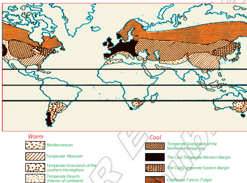
Figure 2.58 Natural regions of the temperate zone
